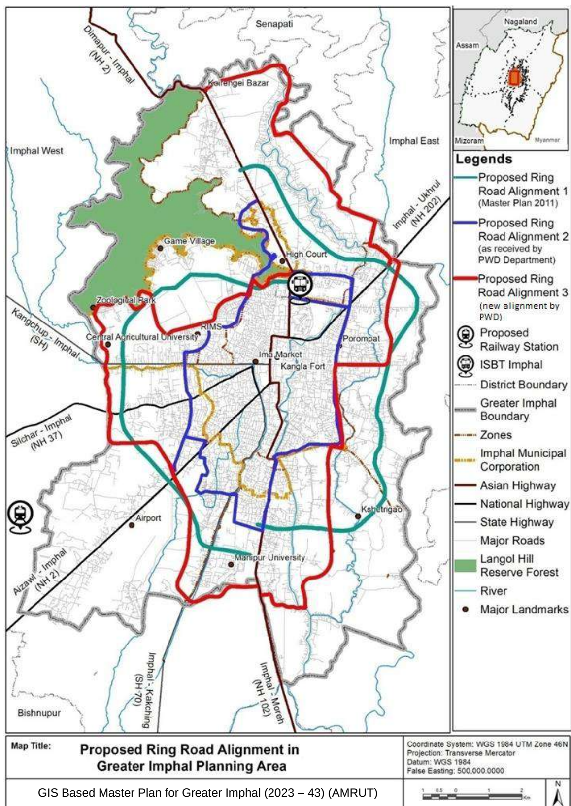
Map 8. 10: Proposed Ring Road Alignments within Greater Imphal planning area
