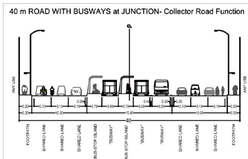
Figure 15. 7: Suggested urban road cross sections
