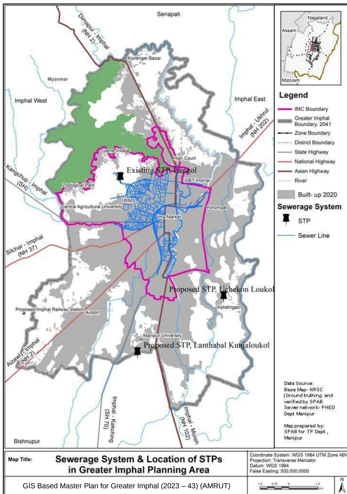
Map 10. 3: Sewerage Network in Imphal Municipal Corporation
