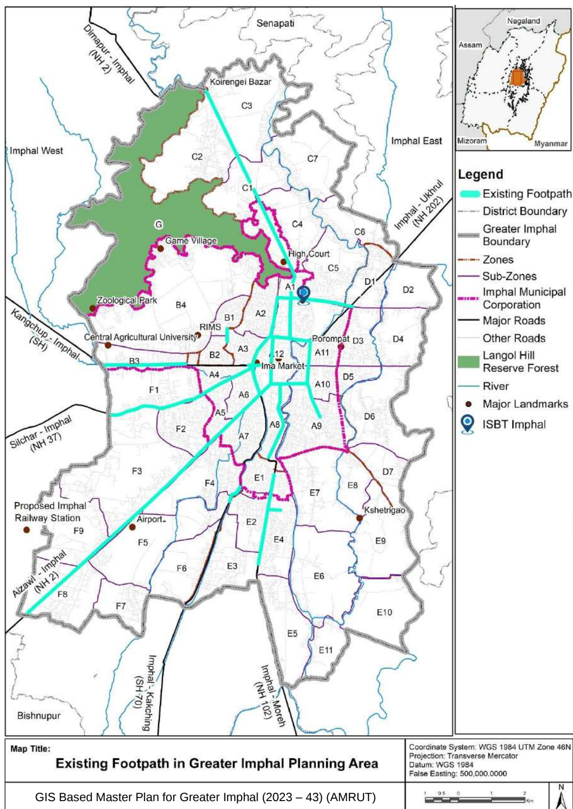
Map 8. 17: Existing Footpath in Greater Imphal Planning Area
