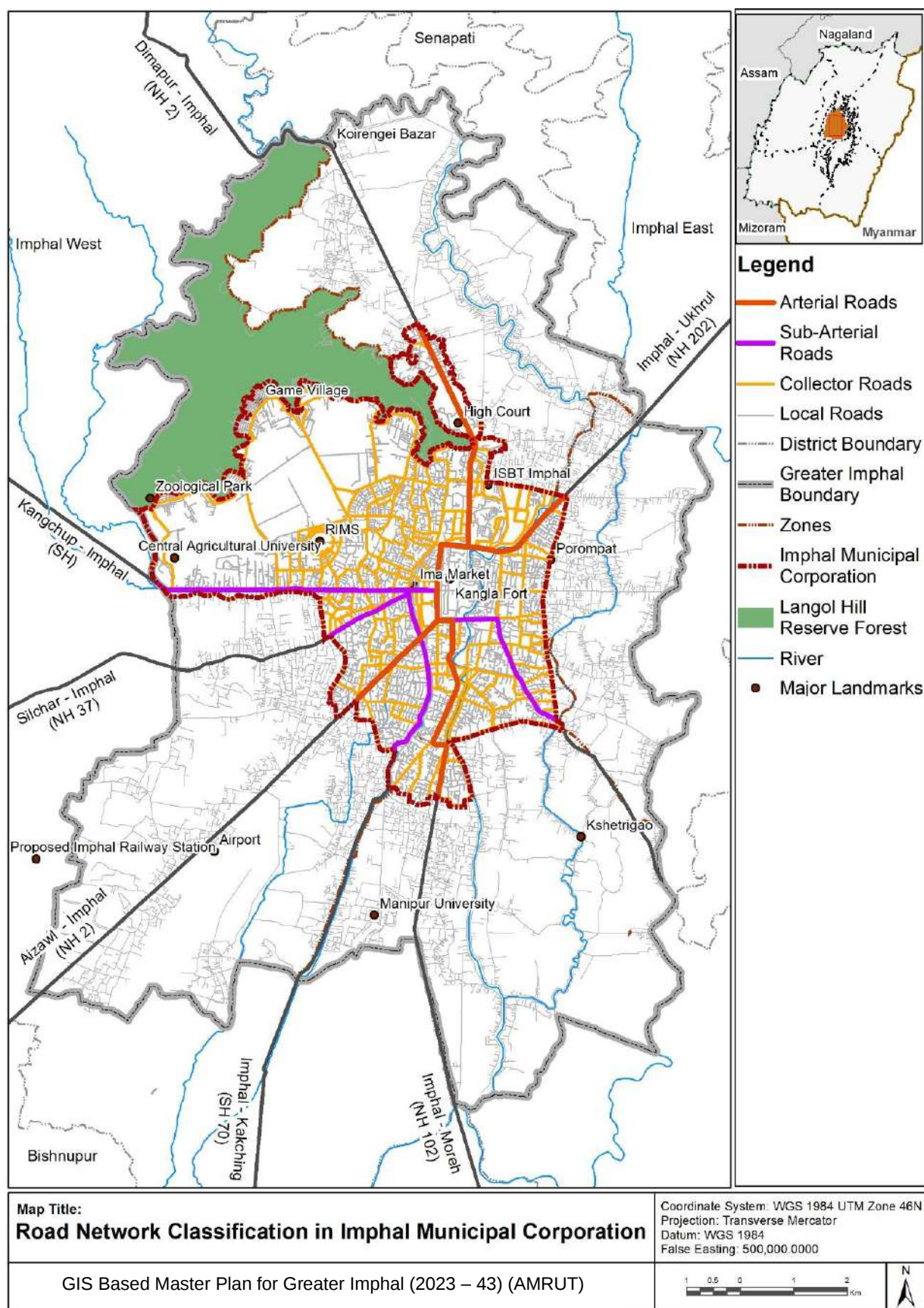
Map 8. 3: Road Network Classification in Imphal Municipal Corporation
