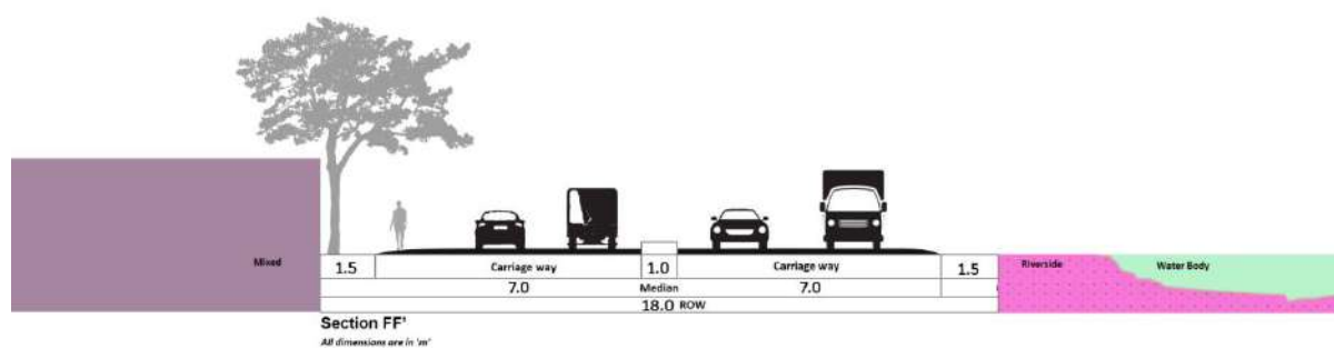
Figure 8. 2: Selected sub-arterial road cross sections in Greater Imphal Planning Area
